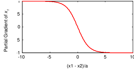
Fig. 4. Partial wirelength gradient for x_1 as a function of (x_1 - x_2)/\alpha .
