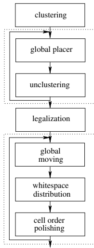
Fig. 1. The outline of our placement flow.
