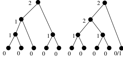
Fig. 3. A multi-level clustering hierarchy, with a clustering ratio of 2 and a required final target number of clusters equal to 2. Each node is labelled with its position in the clustering hierarchy.
