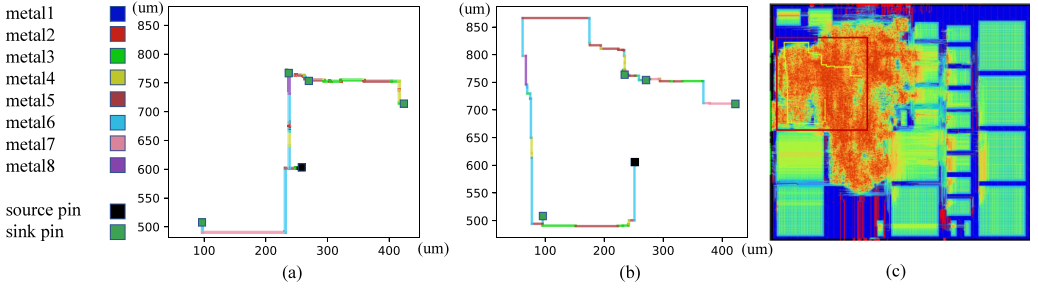
Fig. 5. Differences between the GR guides and post-DR routes of a 5-pin net from swerv_wrapper 45nm. (a) Route guides in post-GR. (b) Post-DR routes. (c) Net highlighted in congestion map.
