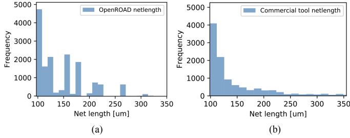
Fig. 12. Wirelength distribution of swerv_wrapper 45nm: (a) for a design with size of 1.20 \times 1.09\text{mm}^2 generated in OpenROAD, and (b) for a design with size of 1.18 \times 1.18\text{mm}^2 generated in a commercial tool flow.
