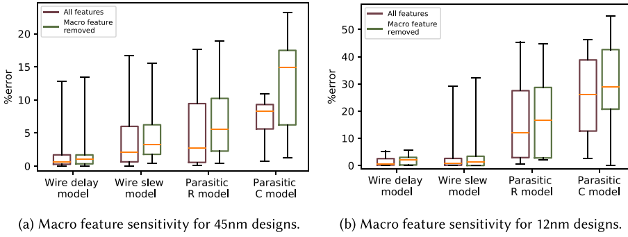
Fig. 10. Macro feature sensitivity for nets that have a region with >80% blockage in their bounding box.
